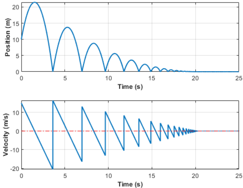
Simulation Results Using Adaptive Zero-Crossing Algorithm
