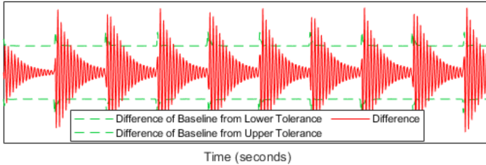
Actuator Model - ode1 (11 signals out of tolerance) - Difference
