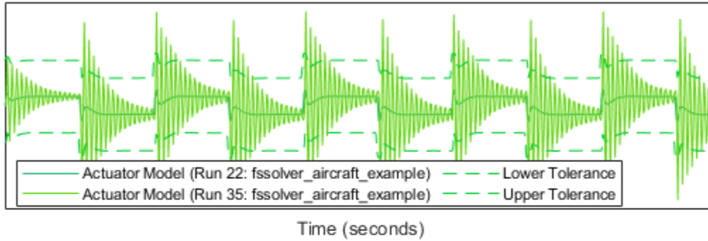
Actuator Model - ode1 (11 signals out of tolerance) - Tolerance
